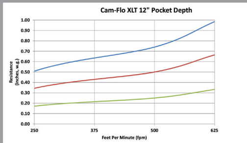
Resistance versus Airflow ■ MERV 14 ■ MERV 13 ■ MERV 11
